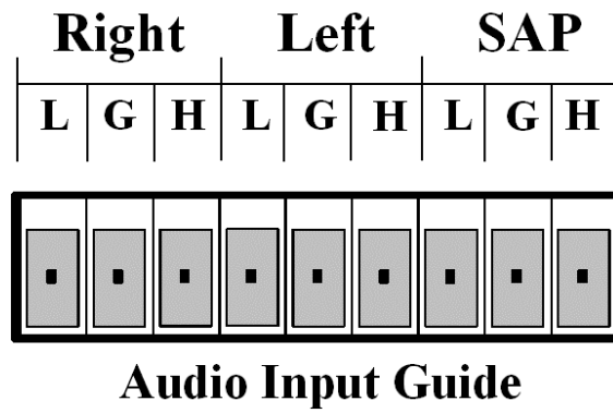
Figure 1.1b Rear Panel Audio Layout of the M369SS Agile Modulator
